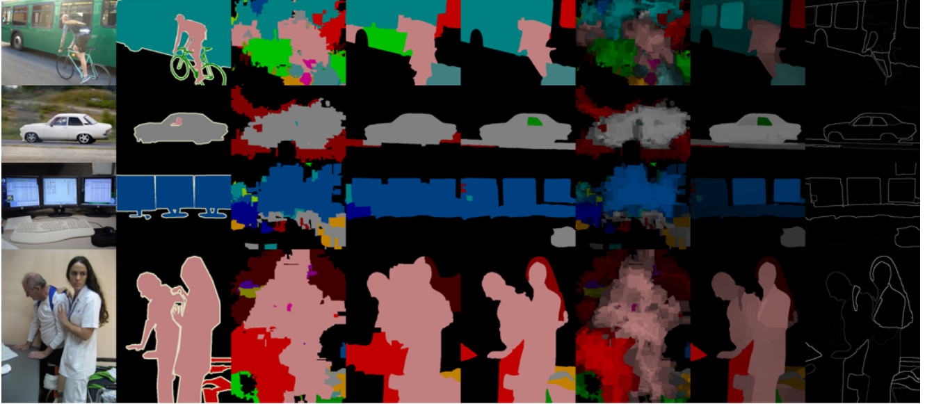
Figure 2. Examples of segmentation on Pascal VOC 2007 data set. Images on each line starting from left to right are respectively: the original image, ground truth segmentation, results of local classifier, CRF and herding, results with intensity proportional to the posterior probability of the local classifier and herding, and the herding estimate of the pairwise probability of the existence of a boundary (the corresponding posterior probability for CRF cannot be easily obtained). Neighboring superpixels of a distance up to 3 hops are used for training local SVM. Best viewed in color.
